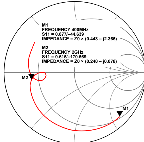
Figure 62. S11 of ADL5521 with S22 Matched at 2 GHz
